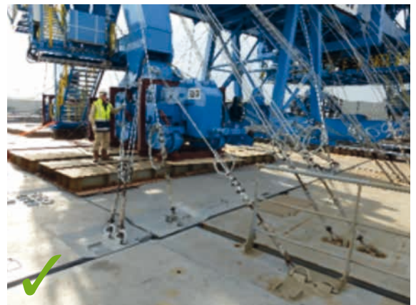
Lashing wires with sufficient scope and clear working space.
